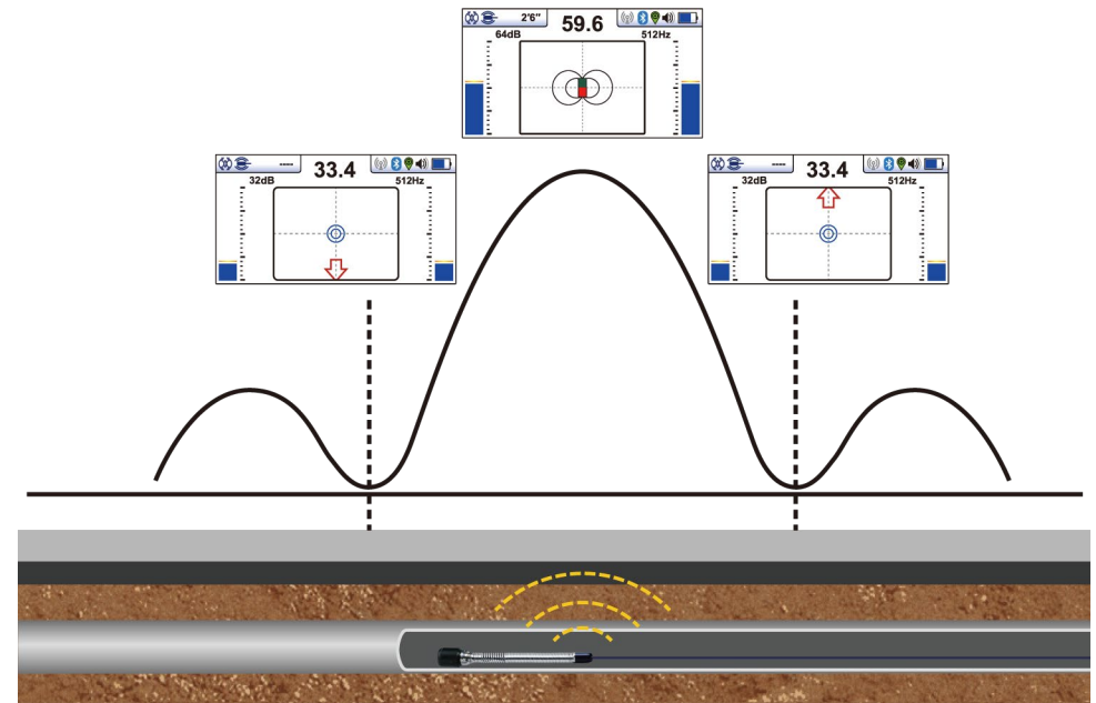
Receiver display
